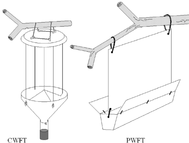
Figure 1. — Design of two window-traps offering an interception area of 1 m 2 : a cross-vanes window flight trap (CWFT) and a single-plane window flight trap (PWFT)
